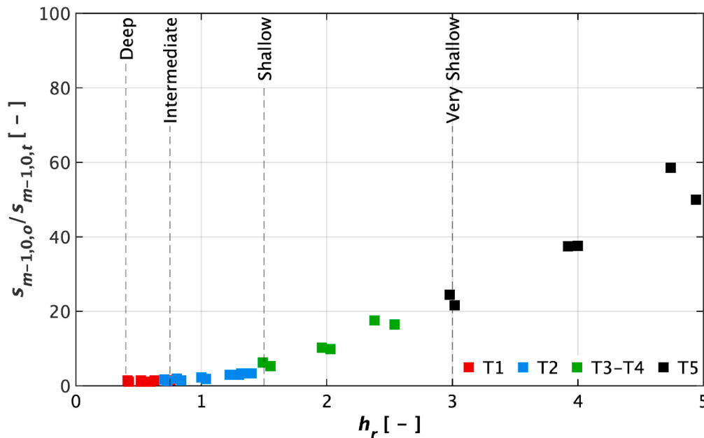
Fig. 9. Influence of the relative depth on s_{m-1,0,o}/s_{m-1,0,t} for different shalowness conditions.
