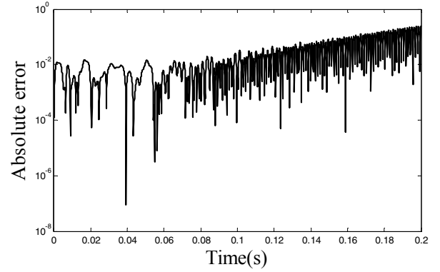
Figure 6. Logarithmic error between the full system and the reduced system.
