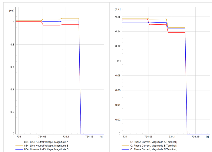
Figure 15. DG trip event ( \mu PMU5).
