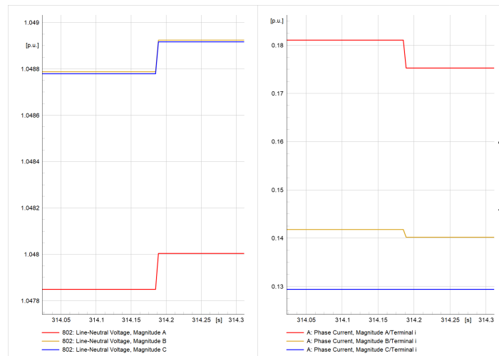
Figure 14. DG switch-off event ( \mu PMU1).
