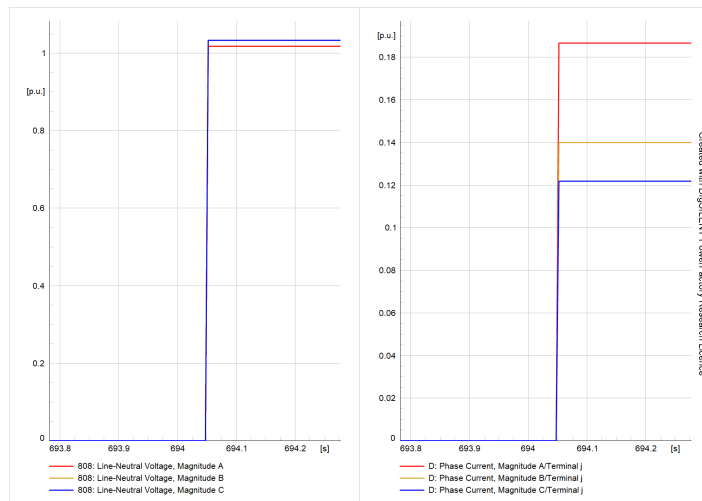
Figure 20. Line section energization ( \mu PMU2).
