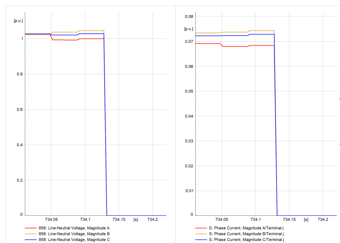
Figure 16. DG trip event ( \mu PMU6).
