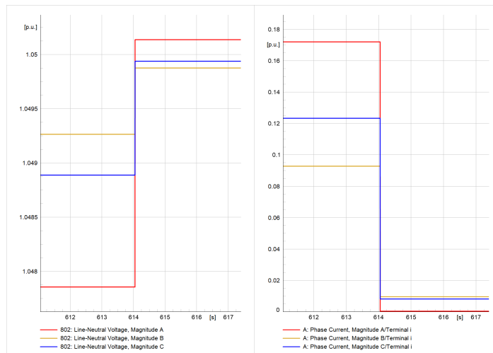
Figure 17. Line section de-energization ( \mu PMU1).
