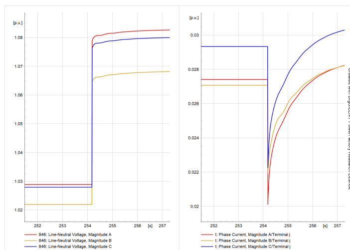
Figure 22. ABCN load switch-off event ( \mu PMU11).
