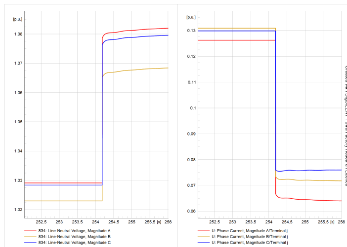
Figure 21. ABCN load switch-off event ( \mu PMU7).
