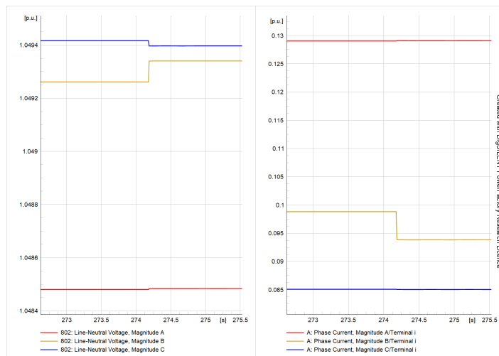
Figure 27. B-N jumper parted open circuit fault (µPMU1).
