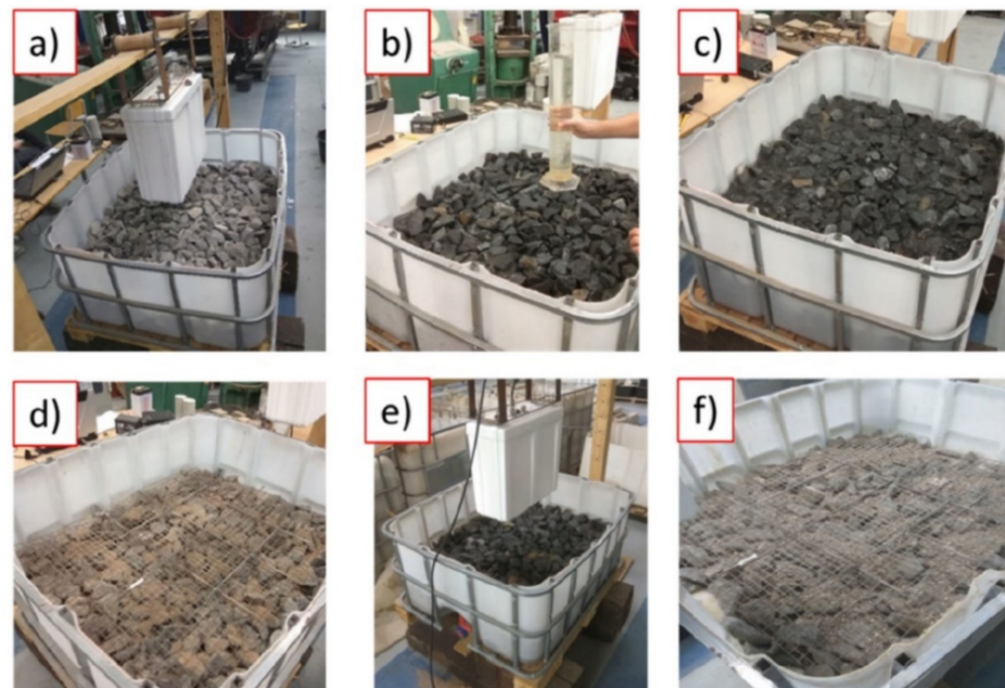
Figure 10. (a–f) demonstrate the whole testing procedure, including test set-up, test conditions and GPR positions. Test configurations of ballast box with ballast particles and fouling (figure reproduced from [63]).
