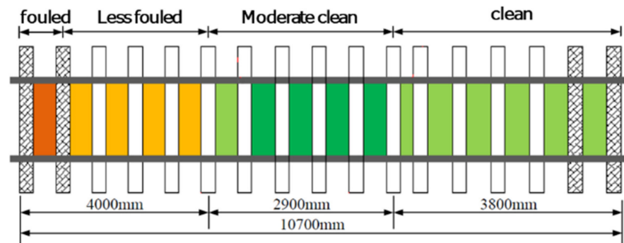
(a) Ballast fouling conditions of track model
