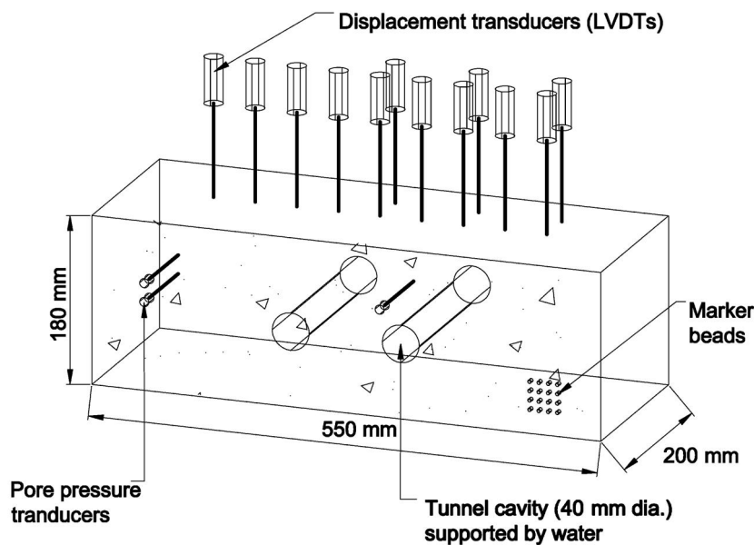
Figure 2: Schematic diagram of a typical plane strain centrifuge twin-tunnel model (not to scale)
