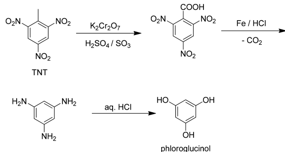
Scheme 1. Phloroglucinol Manufacture before 1980
