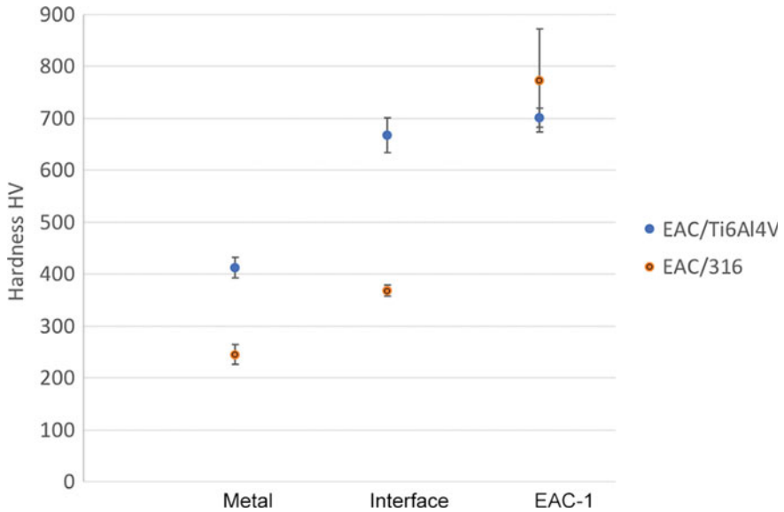
Fig. 4.16 Vickers hardness profile of the functionally graded multimaterials
