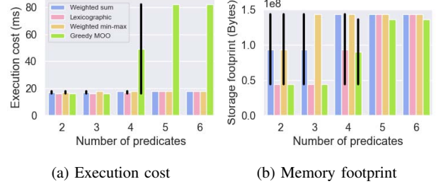
Fig. 4: Query plan performance for the OD scenario
