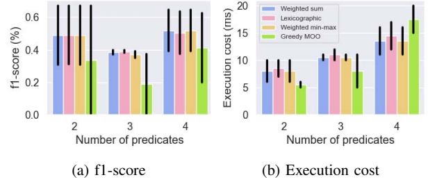
Fig. 3: Query plan performance for the NLP scenario
