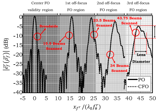
Fig. 9. Normalized electric field in the focal plane of the parabolic reflector when scanning 0 (broadside), 15.5, 23.5, 34, and 43.75 beams. The shaded regions represent the FO applicability regions. The edge taper level of the field intercepted by a lens element is also shown as an example.
