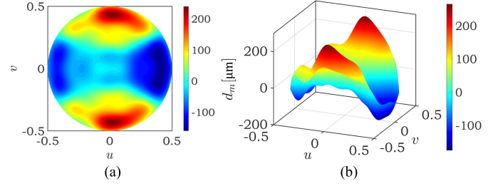
Fig. 13. Shaping the surface of the lens element scanning 43.75 beams. (a) Zernike expansion of the phase needed to be compensated, i.e., the hologram phase. (b) Required modification on the lens surface.
