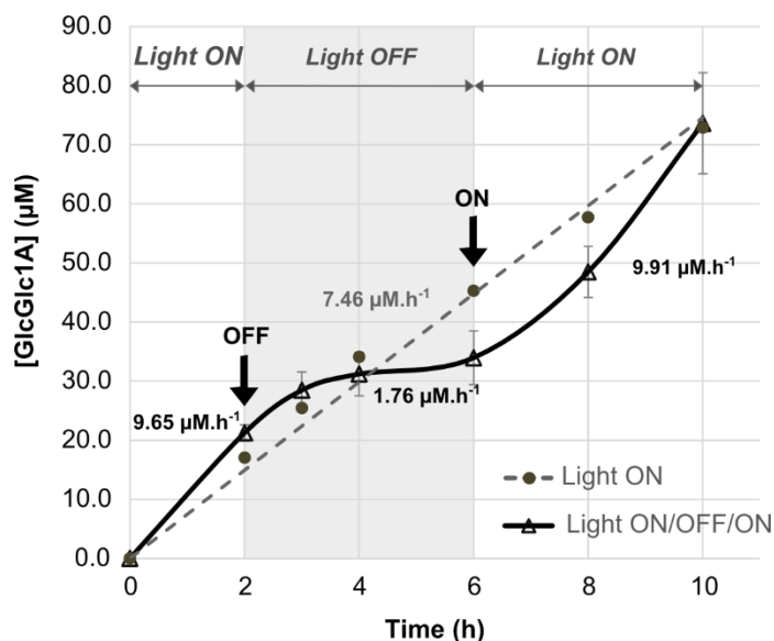
Figure 3 | Impact of a light/dark cycle on the h\nu/V\text{-TiO}_2/\text{LPMO} photobiocatalytic system. The figure shows a time-course for oxidation of Avicel ( 10 \text{ g.L}^{-1} ) by ScLPMO10C ( 1 \text{ μM} ) in the presence of V\text{-TiO}_2 ( 5 \text{ g.L}^{-1} ). Before quantification, soluble products were hydrolyzed by TfCel5A , yielding oxidized products with a degree of polymerization of 2 or 3 ( \text{GlcGlc1A} , (\text{Glc})_2\text{Glc1A} ). Reactions were carried out in sodium phosphate buffer ( 50 \text{ mM} , \text{pH } 6.0 ) at 40 \text{ °C} under magnetic stirring and exposed to visible light at an intensity of 25% of maximum intensity (approx. 42 \text{ W.cm}^2 ). Derived cellobionic acid release rates are plotted on the graph for each light phase (9.65, 1.76
