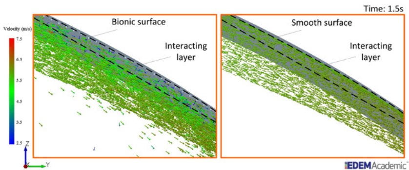
Figure 7.10: Particle velocities of the interaction layers on the bionic surface (group 2) and smooth surface
