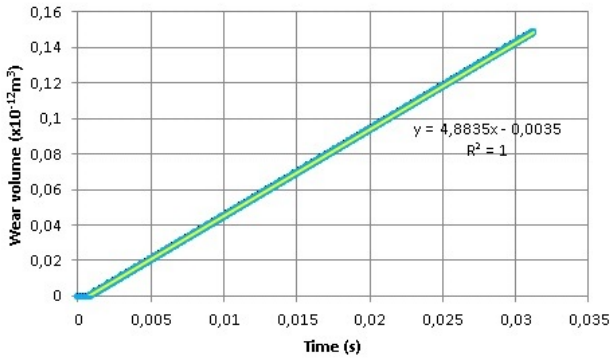
Figure 5.12: Wear volume as a function of time at the early stage
