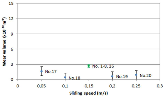
Figure 4.21: Wear volume of mild steel as a function of sliding speed
