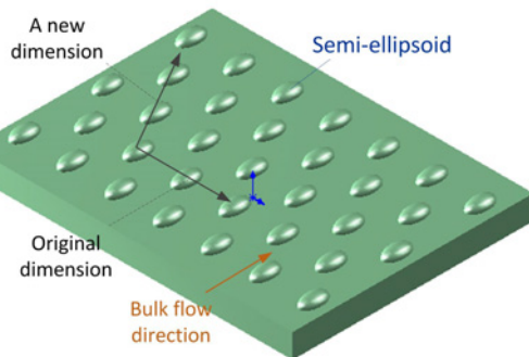
Figure 3.15: Bionic model for abrasive wear reduction
