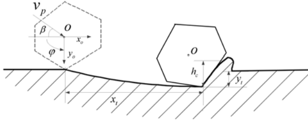
Figure 2.15: Cutting wear model of single particle impact based on [53]
