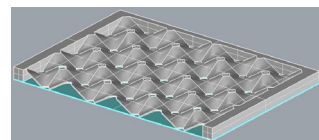
Figure 18: Overview of the thin glass composite panel with 3D printed perforated hyper-shaped core [Akilo, 2018]
