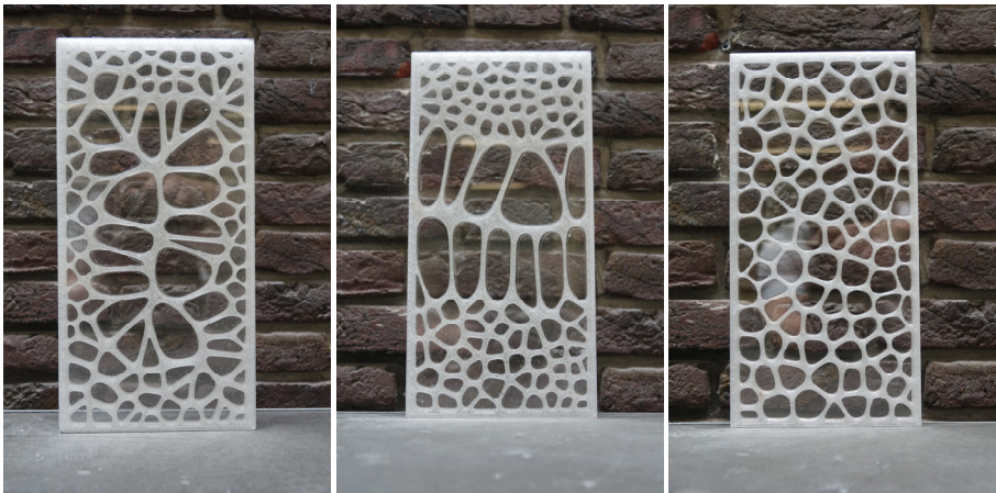
Figure 20: Thin glass panels with 3D-printed PETG Voronoi core patterns [Neeskens, 2018]
