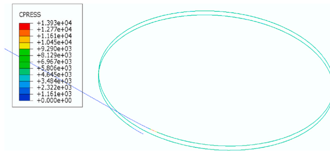
Fig. 28. Contour plot of CPRESS along the path.
