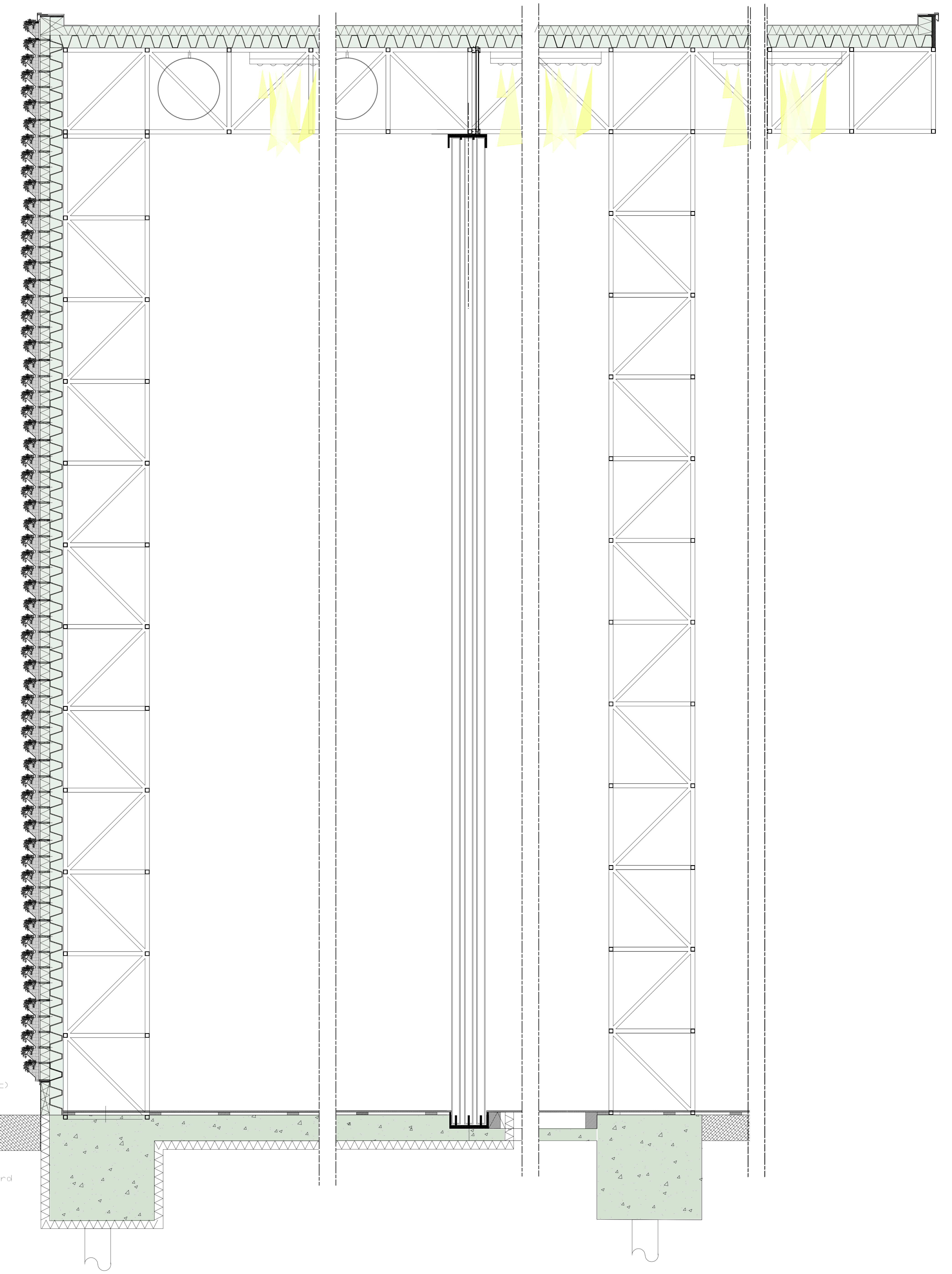
doorsnede trainingshal 1/20 + details 1/10
