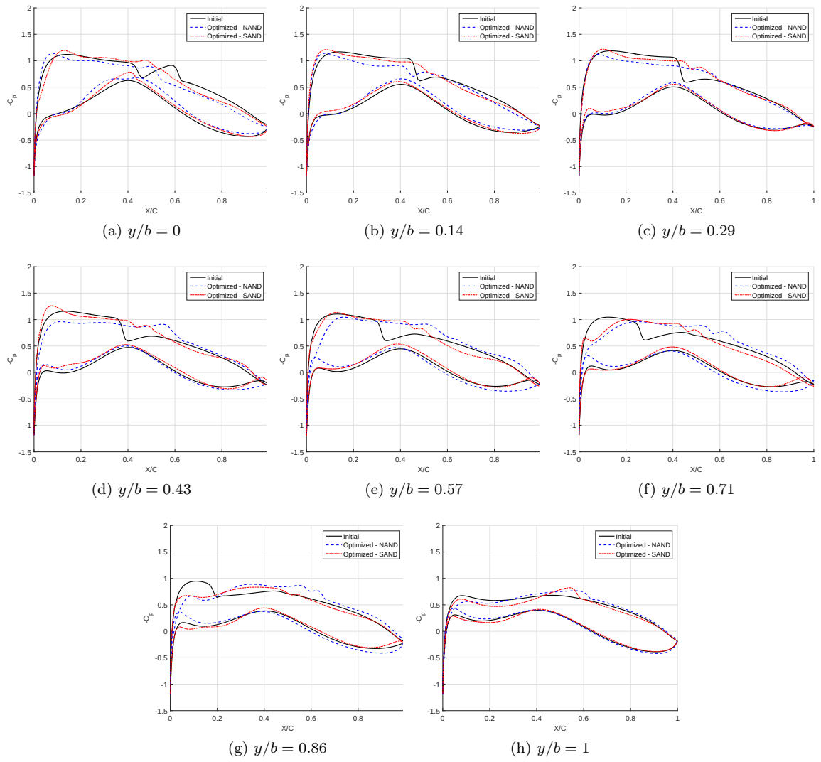
Figure 10: Pressure distribution on airfoils in several spanwise positions.
