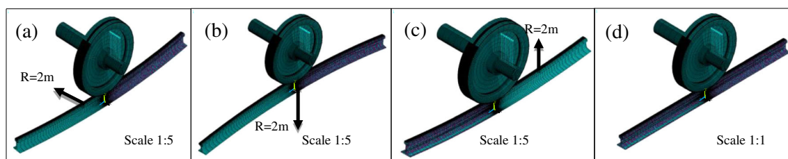
Fig. 4 3D FE models of the wheel–rail contact in different alternatives, a Alt-1, b Alt-2, c Alt-3 and the actual railway as the reference case d; arrows with R = 2\text{ m} show directions of the rail curvature in different cases
