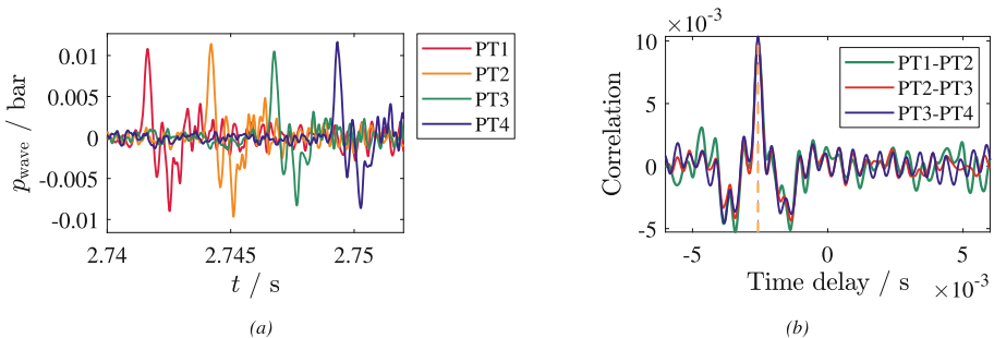
Fig. 3. (a) Over-pressure recording of a small-amplitude wave by sensors PT1 to PT4 (b) Output of cross-correlation technique showing a peak at time-delay between sensors
