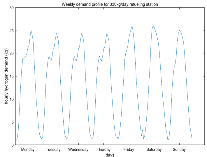
Figure 6: Hourly hydrogen demand profile for an entire week
