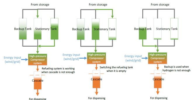
Figure 8: Control logic for the refueling
