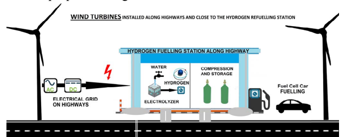
Figure 1 : System overview of on-site wind powered hydrogen refueling station
