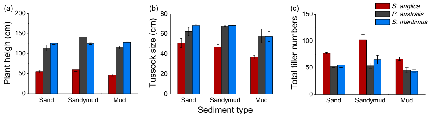
Fig. 3. Plant trait responses found in mesocosm experiment 1 of three marsh species (see Fig. 2 for full names) grown in three contrasting sediment types: Sand, sandy mud, and mud. The response parameters measured were (a) plant height (cm), (b) tussock size measured as maximum distance between expanded tillers (cm), and (c) Total number of tillers per mesocosm of 0.28 m 2 (70 \times 40 cm). See Table 1 for statistical test results.
