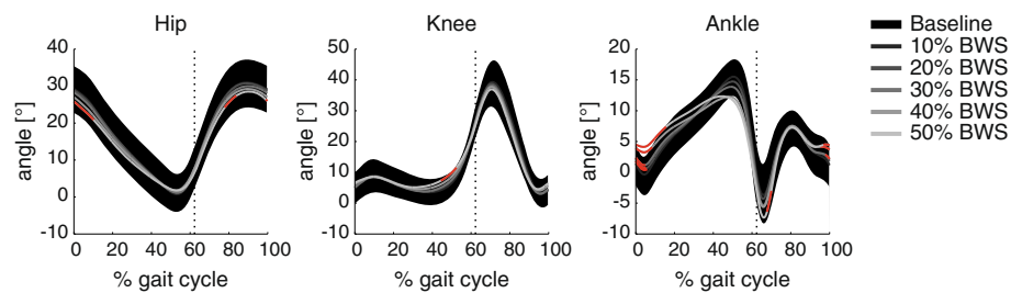
Fig. 2 Angular trajectories of the hip-, knee-, and ankle angle in the sagittal plane during a gait cycle are shown across all levels of unloading (black area shows the \pm 1 standard deviation interval during baseline condition). The time intervals during which significant differences between unloaded condition and baseline were found are highlighted in red. The vertical line indicates the mean time point of toe-off across all levels of unloading. BWS = body weight support
