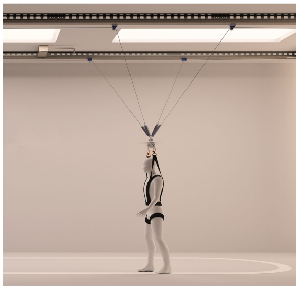
Fig. 1 The cable robot is powered by four motors that actuate a central node via a ceiling-mounted rail- and deflector system. The design of the body weight support system allows unrestricted walking on level ground or on stairs as well as training paradigms such as sit-to-stand transition
