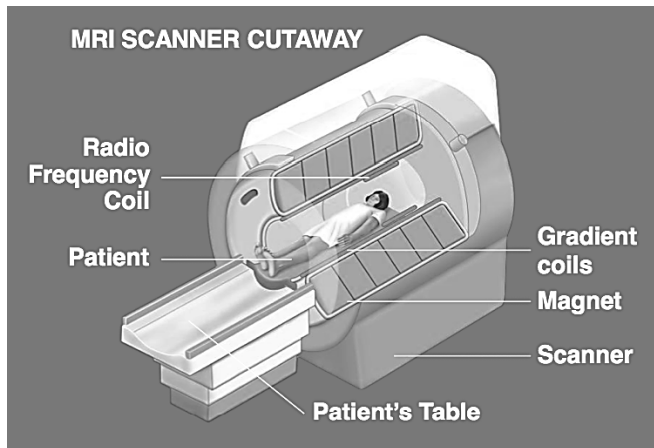
Figure 1.5. Overview MR scanner with special attention to the gradient, RF, and main magnetic field.
