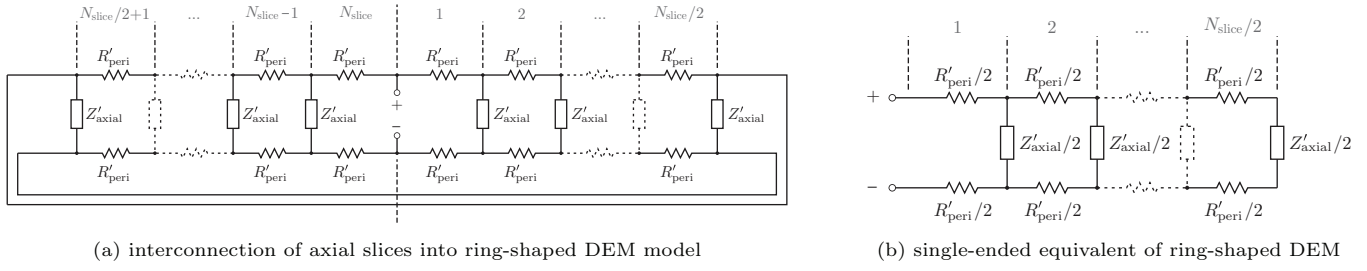
Figure 10. Full DET model by interconnection of axial slices into ring-shaped DEM.
