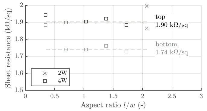
Figure 18. Measured electrode sheet resistance.
