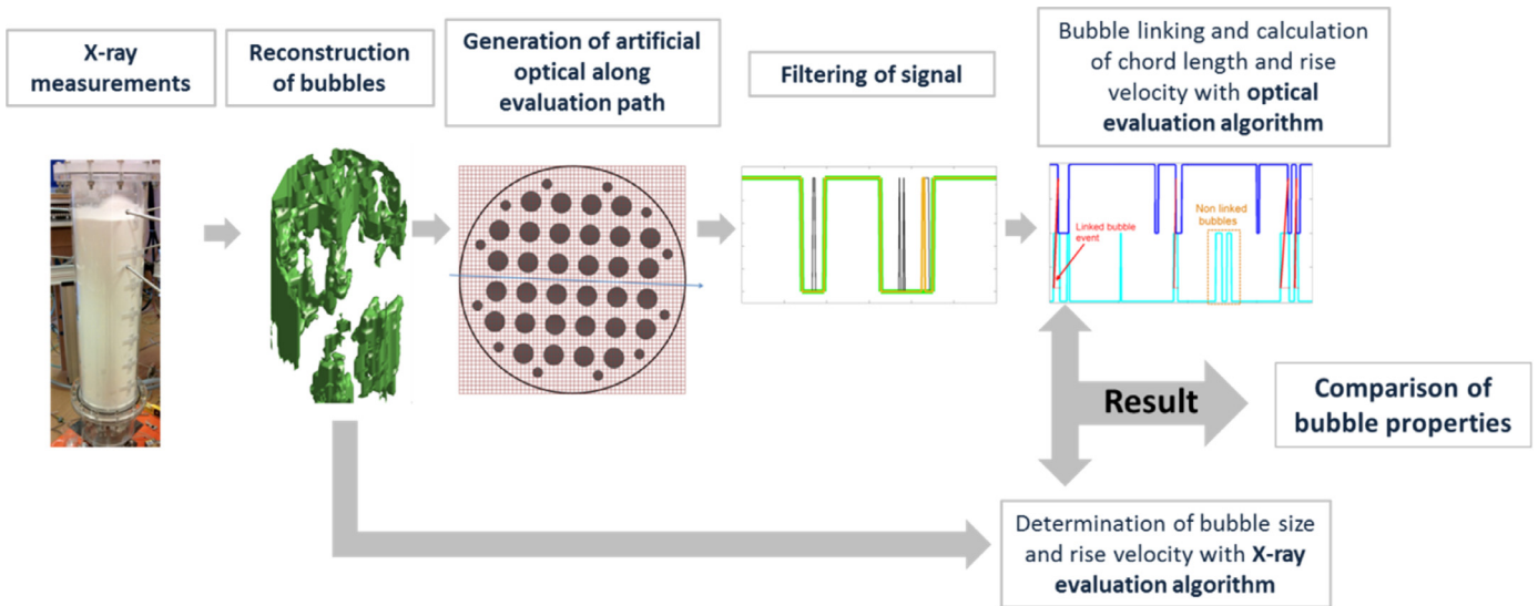
Fig. 9. Data processing scheme.
