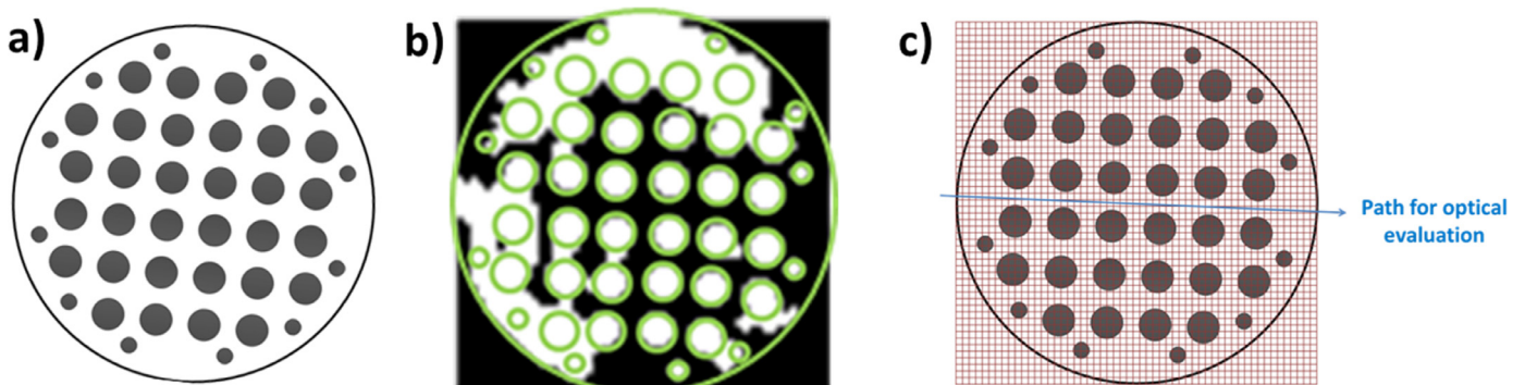
Fig. 3. (a) Cross-section of the column, (b) exemplary reconstructed fluidization state determined by X-ray measurements with overlaid internals, (c) overlaid 55 \times 55 pixel pattern for generation of fictitious optical signal (with evaluation path along the centerline of the column).
