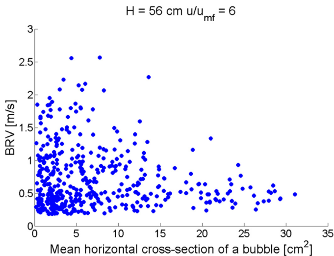
Fig. 16. Scatter plot of BRV and the corresponding mean cross-sectional area for all detected bubbles at a measurement height of 56 cm and a fluidization number of six.
