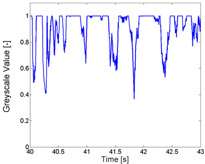
Fig. 6. Signal of grey scale plotted over time for a random pixel in the 55 × 55 patter.
