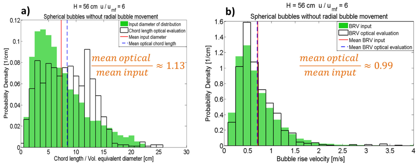
Fig. 24. Comparison of diameter (a) and bubble rise velocity (b) distribution for the input into the MC-simulation with the results generated by the optical evaluation for spherical bubbles.
