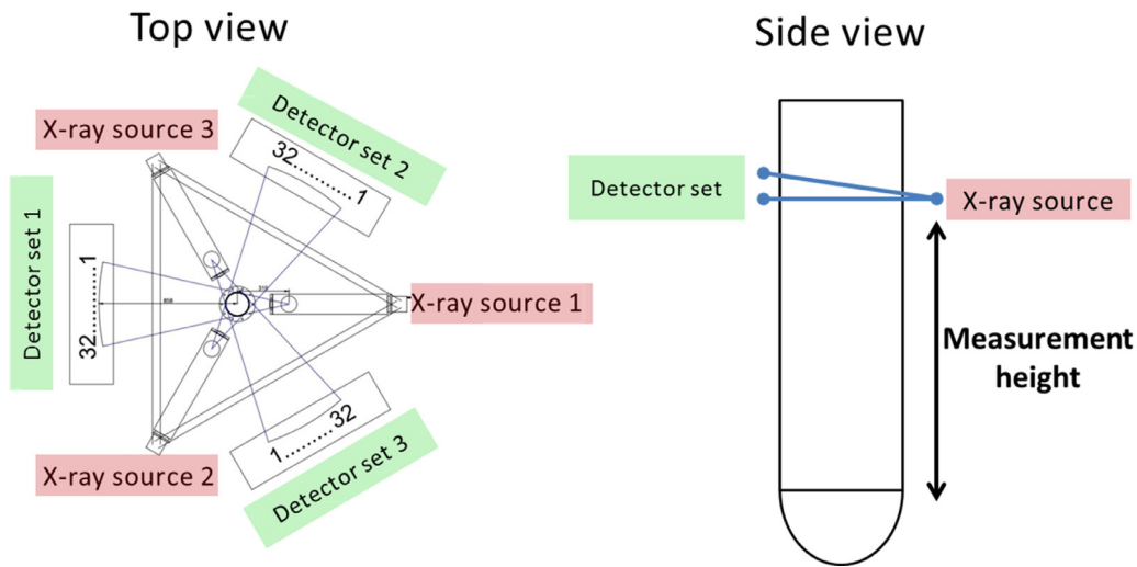
Fig. 4. Top view and side view of the X-ray tomographic setup adapted from (Maurer et al., 2015c).
