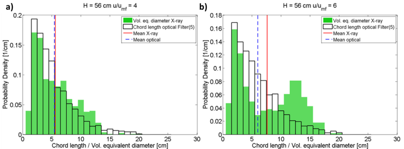
Fig. 20. Histograms of the chord length distribution for the filtered artificial optical signal and the volume equivalent diameter (above the entire cross-section) for the X-ray evaluation at H=56\text{cm} and u/u_{mf} of 4 and 6.
