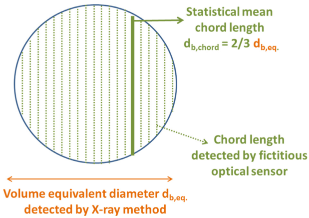
Fig. 19. Visualization of mean chord length for a bubble pierced at various positions by the fictitious optical sensor and the volume equivalent bubble diameter (X-ray method).
