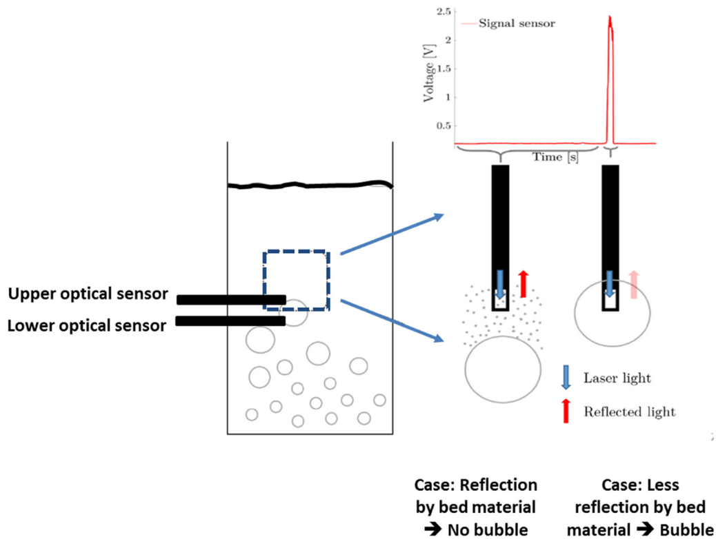
Fig. 1. Measurement principle of the optical sensor.
