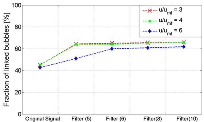
Fig. 11. Influence of filter strength on annulus weighted (see Section 5.2) fraction of linked bubbles for a measurement height of 56 cm.
