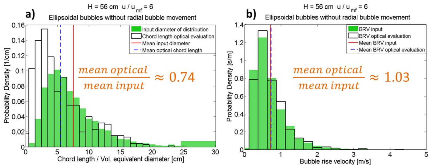
Fig. 25. Comparison of diameter vs. chord length (a) and bubble rise velocity (b) distribution for the input into the MC-simulation with the results generated by the optical evaluation for ellipsoidal bubbles.
