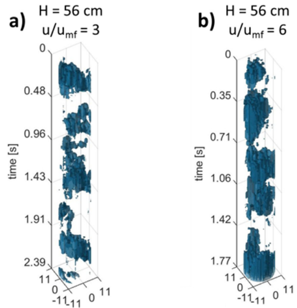
Fig. 21. Reconstructed bubbles at H=56\text{cm} for fluidization numbers of 3 and 6 based on X-ray measurements.
