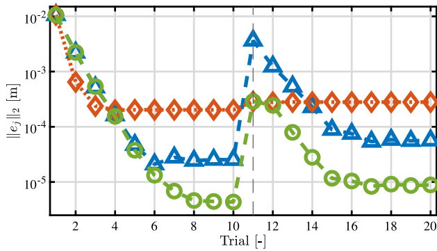
Fig. 8. Error 2-norm for 20 trials of frequency-domain ILC ( \blacktriangle ), basis function ILC ( \blacklozenge ) and developed combined frequency-domain and basis function ILC ( \blacklozenge ). At trial 11, the reference signal is changed (---).
