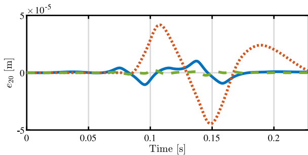
Fig. 9. Tracking error after 20 trials e_{20} of frequency-domain ILC ( \text{—} ), basis function ILC ( \text{---} ) and developed combined frequency-domain and basis function ILC ( \text{- -} ).
