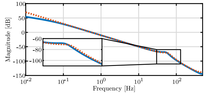
Fig. 10. FRFs of system \mathcal{P}(e^{j\omega}) ( \text{—} ) and of estimate using the inverse basis function feedforward filter \mathcal{F}_{BF}^{-1}(e^{j\omega}, \theta_j) ( \text{---} ), with finite-time representation \mathcal{F}_{BF}(\theta_j)r = \psi\theta_j .
