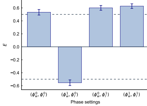
Figure 4.4: Bell test. The values of the correlation coefficients E grouped for the four ideal phase settings of the CHSH inequality, which are (\phi_w^0, \phi_r^0) = (\phi_0 - \pi/4, 0) , (\phi_w^1, \phi_r^0) = (\phi_0 + \pi/4, 0) , (\phi_w^0, \phi_r^1) = (\phi_0 - \pi/4, \pi/2) and (\phi_w^1, \phi_r^1) = (\phi_0 + \pi/4, \pi/2) . The total number of events for each phase setting is \sim 400 . The dashed lines are the threshold for each correlation coefficient to violate the inequality. From these values we obtain S = 2.32 \pm 0.08 , which violates the inequality by 4 SD. All errors are one SD.
