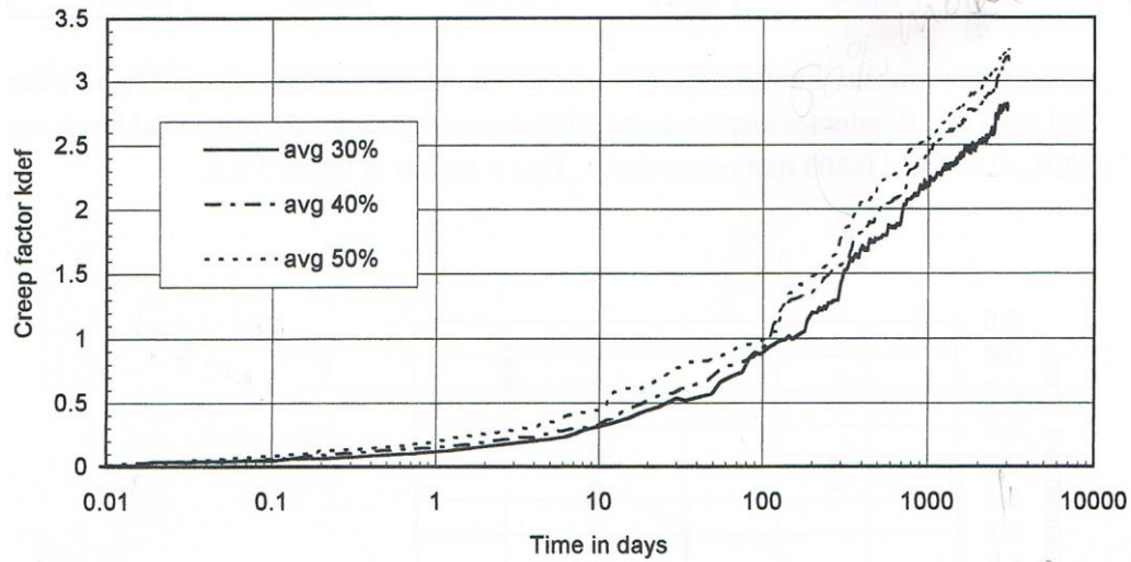
Fig. 7.3.6. Average creep curves of 30%, 40%, and 50% nailed joints
