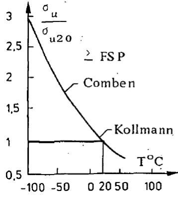
fig. 4.5.3 Saturated wood
