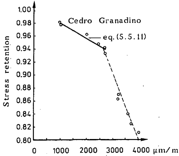
fig. 5.15 Relaxation for compression of tropical wood [9]
