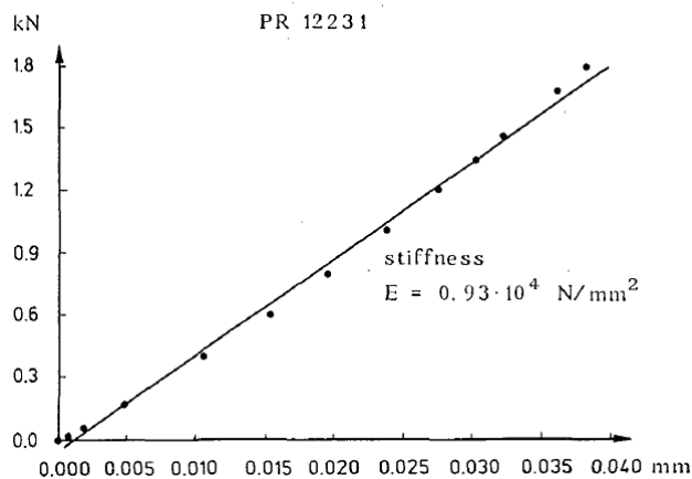
fig. 8.6 First loading of a compression test
