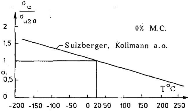
fig. 4.5.4 Dry wood
