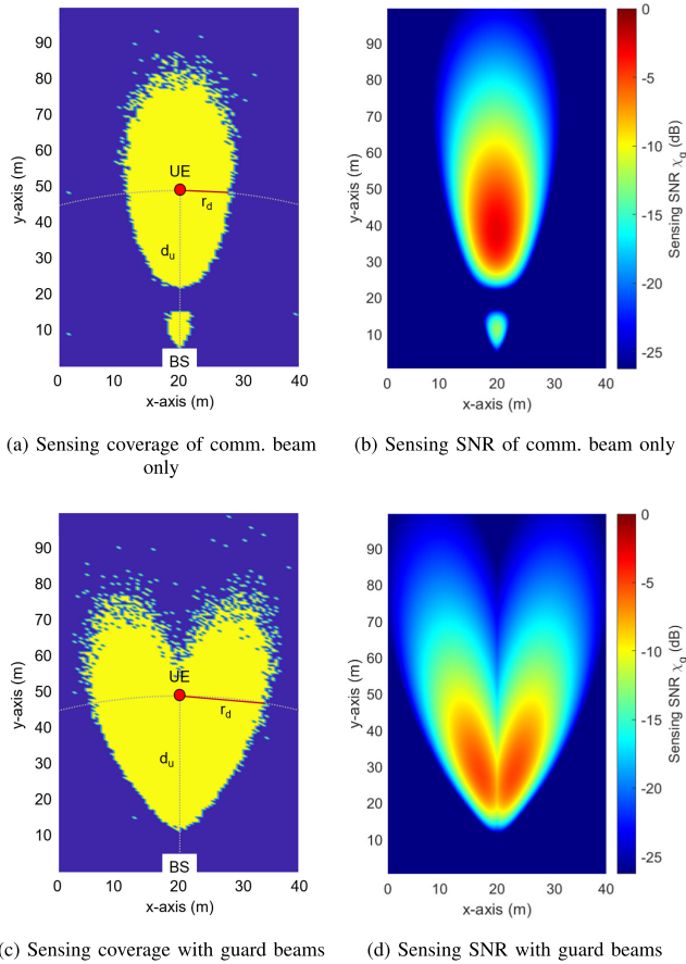
FIGURE 8. Sensing coverage and sensing SNR comparison.
