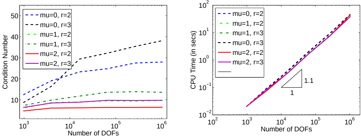
Figure 4: Condition numbers and CPU times for Laplacian with \delta^{sub} = 3h (varying n ).
