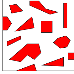
Figure 2: Typical situation for Example 3.2, i.e. “islands” B_k (in red) where \alpha is large.
