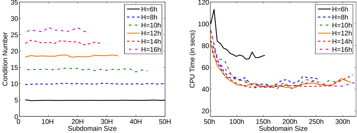
Figure 3: Condition numbers and CPU times for Laplacian with n = 1024^2 , \delta^{sub} = 3h , \mu = 1 .
