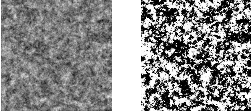
Figure 5: Log-normal and “clipped” log-normal random fields with n = 512^2 and \lambda = 1/64 .
