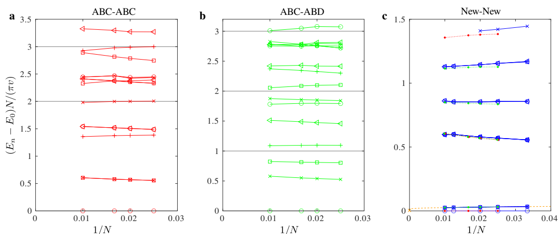
Figure 5: Conformal towers of states of the four-state Potts model with a three-state-mixed symmetric and b three-state-mixed non-symmetric boundary conditions, and c with symmetric boundaries polarized in the direction of the transverse field (following Ref. [24] we use the term "New" boundary conditions). Symbols are DMRG data points extracted from the low-lying energy excitation spectra with velocity v = \pi/4 . Gray lines are integer levels shown for reference. In c the results from a (dotted red) and b (dotted green) are shown as a reference, the latter is shifted such that it starts at the first excited state of the New-New tower. Each level in New-New tower that matches a level of the ABC-ABD tower is three-fold degenerate. Orange dashed line is a finite-size extrapolation assuming log-corrections in the form derived by Cardy [45].
