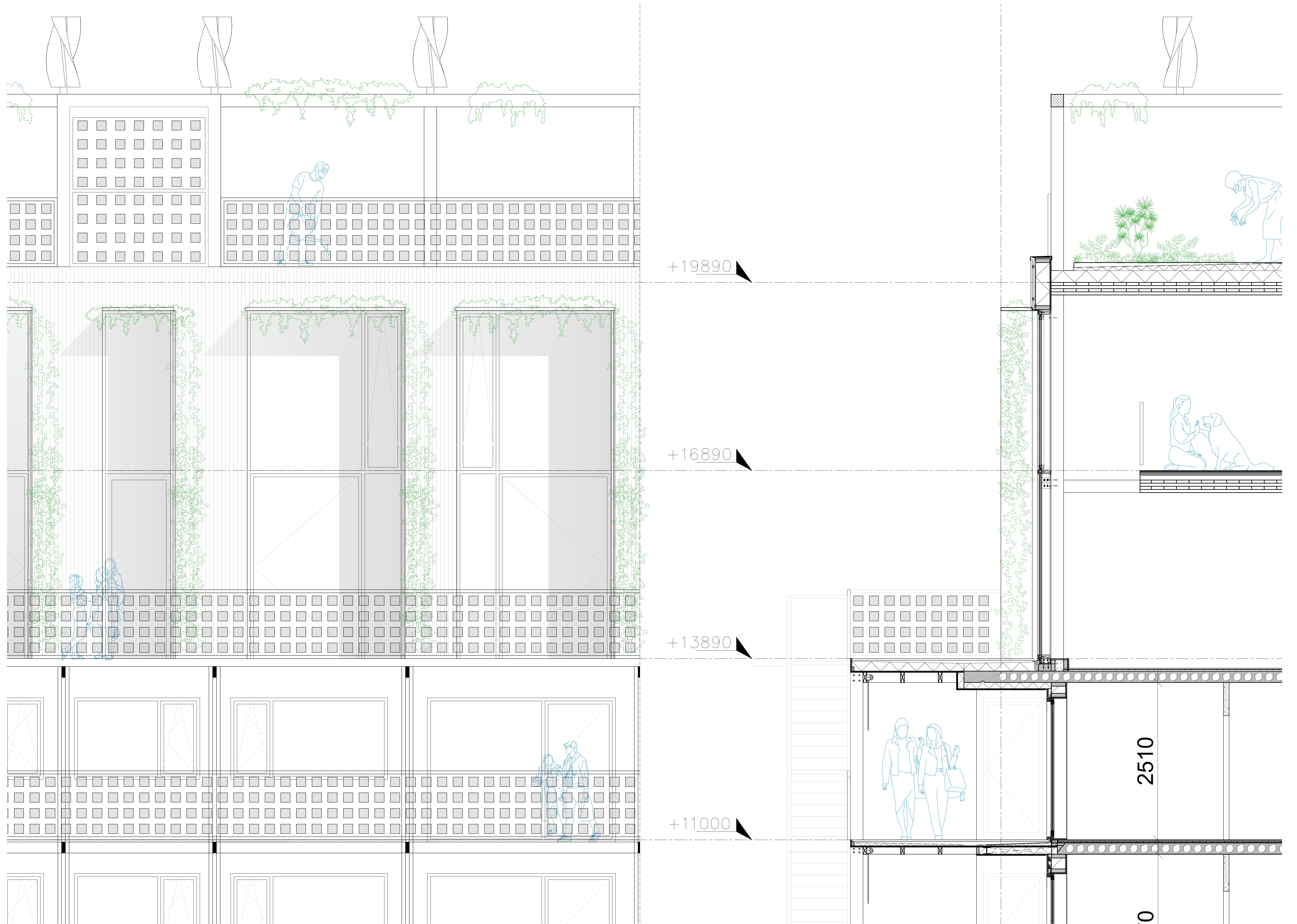
west facade fragment_1:20
