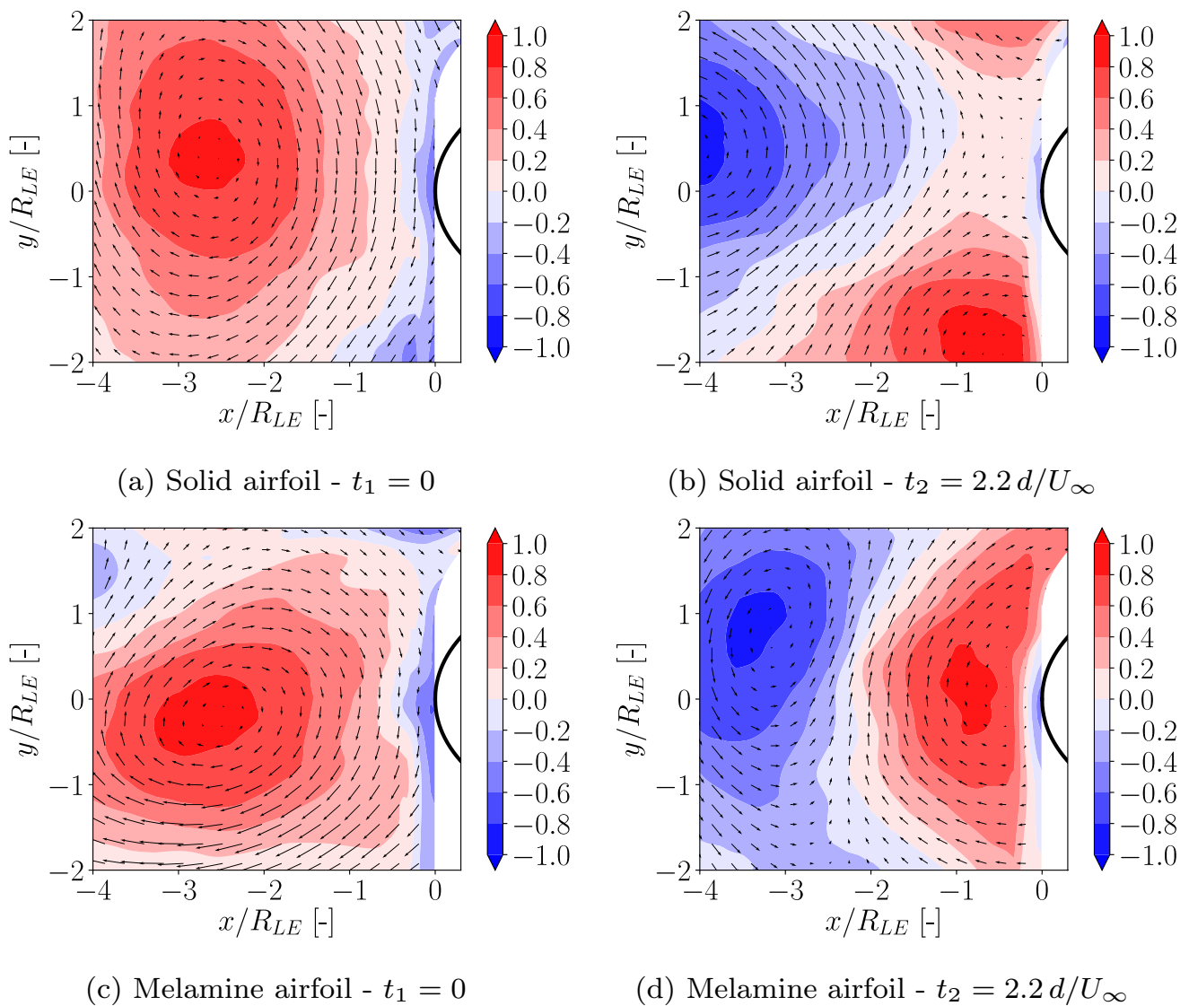
Fig. 15 Instantaneous \Gamma_2 and velocity fields reconstructed with the 0 – 50% POD energy bin for the solid and melamine airfoil models. 14 \times 14 measurement points have been considered in the computation of the function
