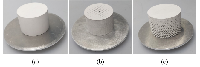
FIGURE 9. Manufactured DRA antennas with different permittivity profiles (a) homogeneous (DRA-H); (b) linear permittivity profile, increasing in the radial direction (DRA-IHR); (c) linear permittivity profile, increasing along the vertical axis (DRA-IHZ).
