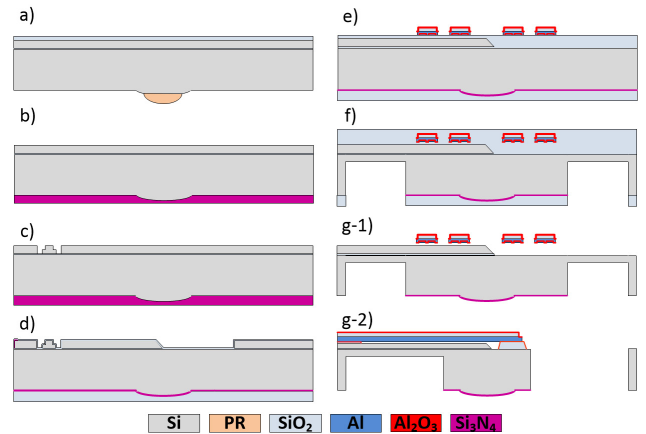
Figure 4: Fabrication process. (a) Shape transfer of reflowed photoresist ball cap to Si using a Si dry etch process. (b) Smoothened microlens with PECVD SiN scratch protection. (c) Two-step waveguide etching process. (d) Mirror etching, sidewall surface roughness reduction, LPCVD SiO 2 cladding, LPCVD SiN antireflecting coating and ALD Al 2 O 3 protective layer. (e) Al-SiO 2 bimorph formation using sputtered Al and PECVD SiO 2 , protected by ALD Al 2 O 3 ; (f) Backside DRIE etching and hinge formation; (g-1): Vertical scanner (g-2): Lateral scanner device release using vapor HF.
