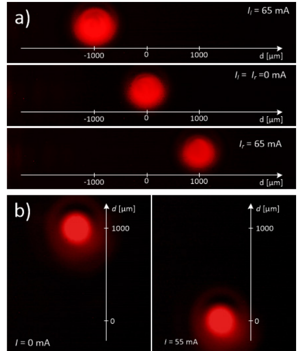
Figure 7: CCD images of MOEMS scanner light spot: (a) lateral scanning direction for (from top to bottom) left side actuated, unactuated and right side actuated light spot. (b) Vertical scanning direction in initial (left) and actuated state (right). The images were postprocessed to introduce false colors and increase the contrast for better visualization of the light spot.
