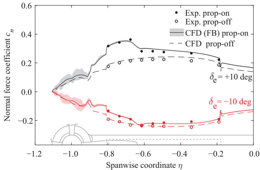
Fig. 11 Spanwise distribution of normal-force coefficient for positive and negative elevator deflection.
