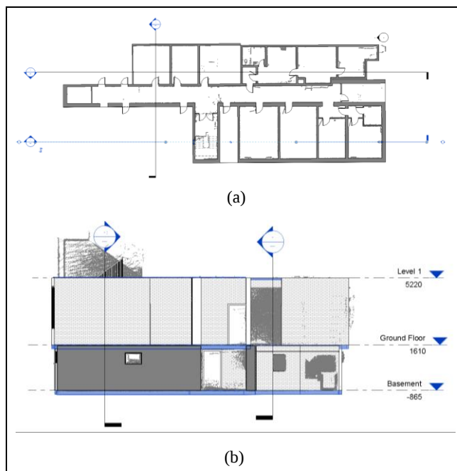
Figure 2. Manual reconstruction of building elements from a point cloud: (a) a horizontal section for the placement of walls, doors and stairs; (b) a vertical section for the placement of floors, ceilings, doors and windows.
