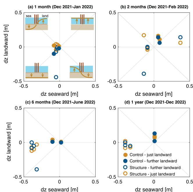
Figure 9. Seabed level changes (dz in meters) measured both landward (vertical axis) and seaward (horizontal axis) of a temporary permeable structure (empty dots), and at a control transect (filled dots) across four different time periods. The diagonal represents equal magnitude of the changes in the seaward and landward points. (a) December 2021–January 2022, representing one month during the Northwest monsoon season; (b) December 2021–February 2022, covering two months of the Northwest monsoon season; (c) December 2021–June 2022, representing a six-month period; and (d) December 2021–December 2022, capturing a full year. These plots illustrate sediment accumulation or erosion patterns in proximity to the temporary permeable structures compared to sites without structures. Sketches illustrating the erosion patterns for different combinations of bed level changes seaward and landward are shown in plot (a).
