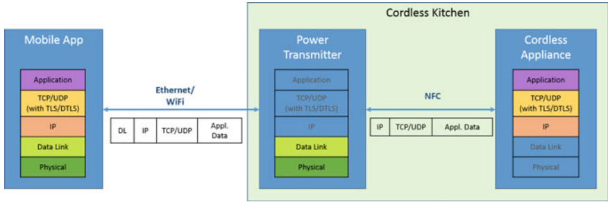
Fig. 3.3 Bridge architecture for Internet connectivity
