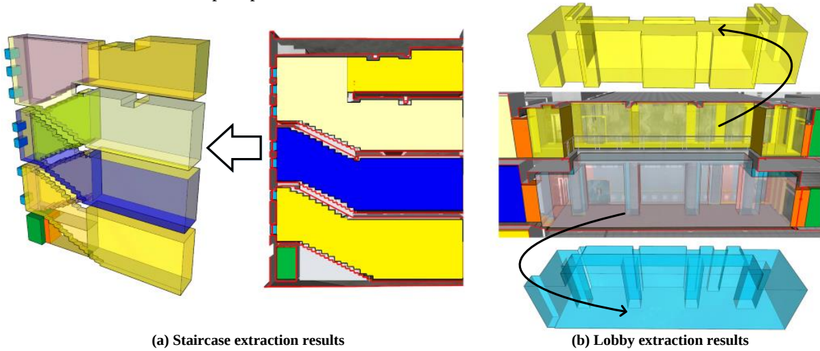
Figure 20 Extraction performance for free multi-floor indoor spaces.
