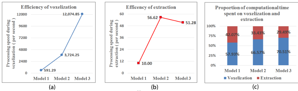
Figure 17 Efficiency comparisons.
