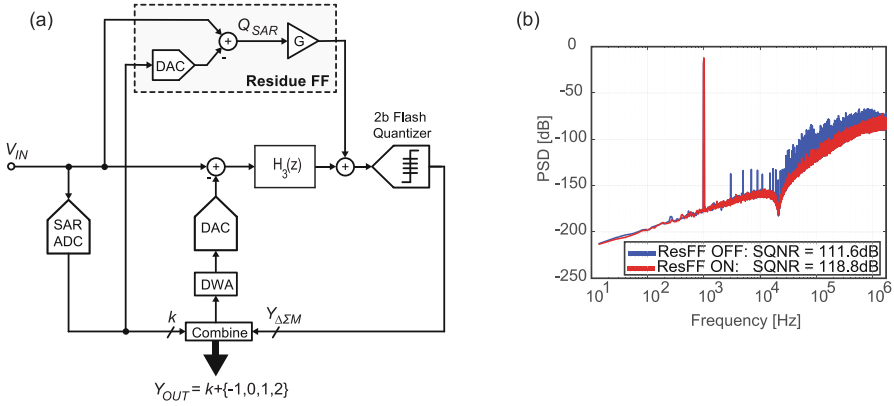
Fig. 6 (a) Block diagram of a zoom ADC with third-order \Delta\Sigma M with 2-bit quantizer, 5-bit SAR ADC, and residue feedforward [1]; (b) Output spectrum of the zoom ADC
