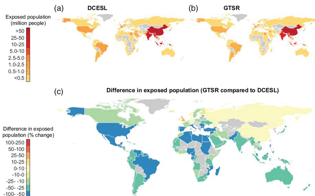
Figure 4. Comparison of exposed population to 1 in 100-year sea levels on a country-scale when based on, (a) DINAS-COAST Extreme Sea Levels (DCESL), and (b) Global Tide and Surge Reanalysis (GTSR), and (c) the difference between exposed population when based on DCESL and GTSR showed as the relative change compared to DCESL (%).
