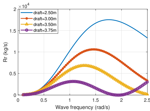
(c) Radiation damping
