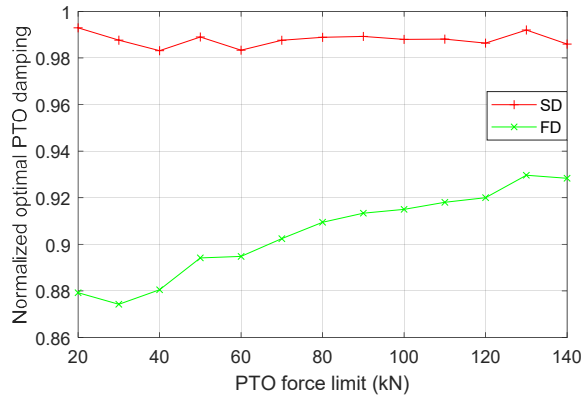
Figure 4.15: The weighted mean values of the PTO damping optimized by the FD and SD modeling normalized to those obtained by the TD modeling.
