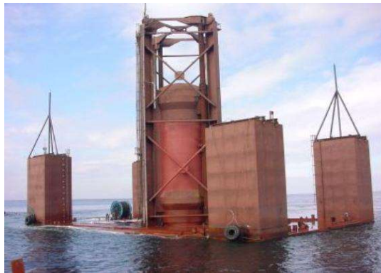
Figure 2.5: AWS WEC [44].
