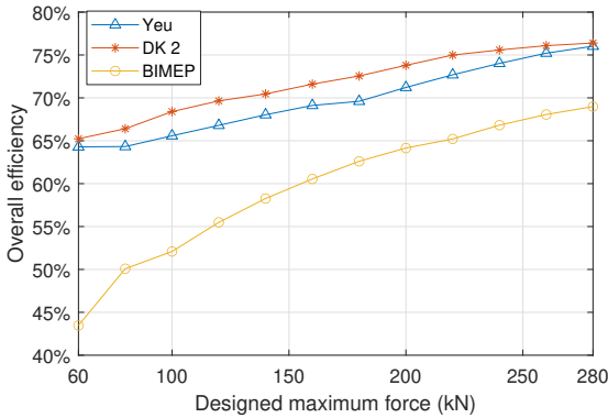
Figure 5.12: The overall efficiency of the linear generator as a function of the designed maximum generator force in different wave sites.
