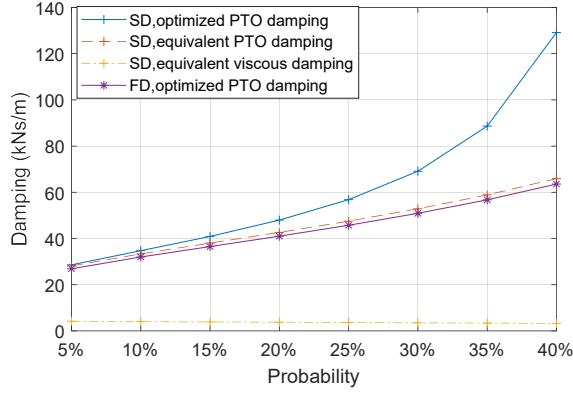
Figure 4.12: The PTO damping coefficients optimized by the FD and SD modeling, the corresponding equivalent PTO and viscous damping in the SD modeling as a function of the allowable probability of the PTO force saturation, H_s = 1.5 m, F_m = 30 kN and T_p = 5.15 s.
