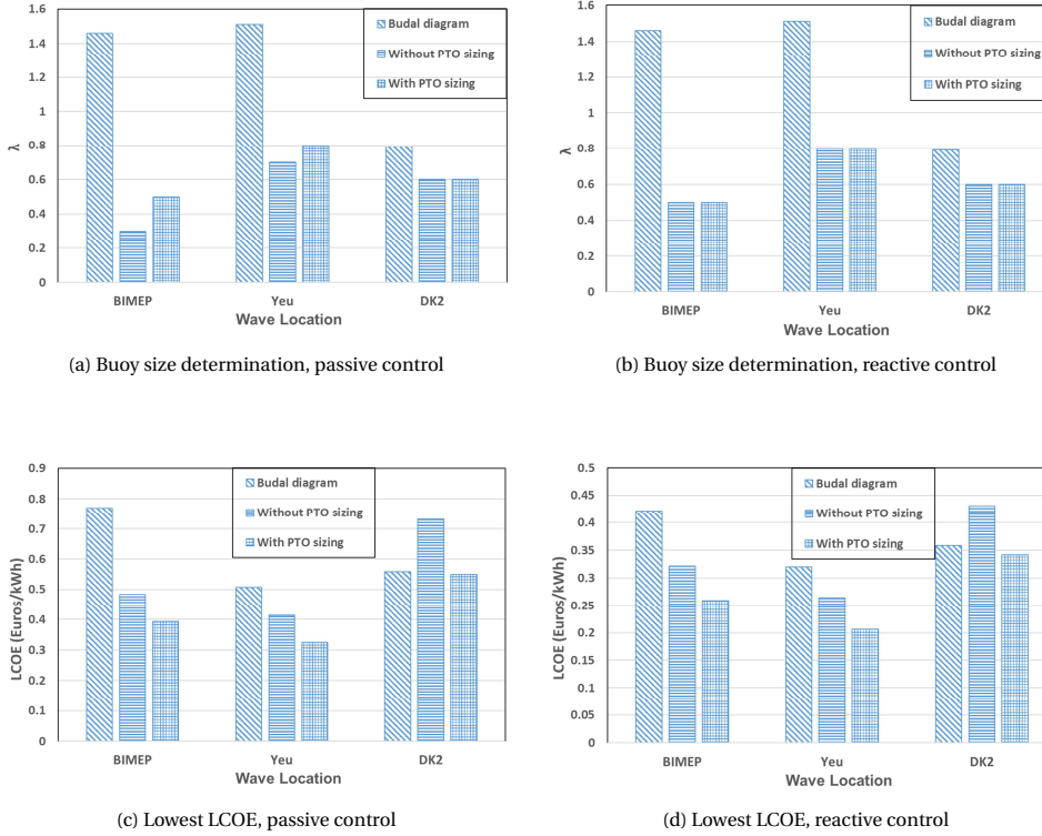
Figure 3.19: Comparison among different size optimization methods.
