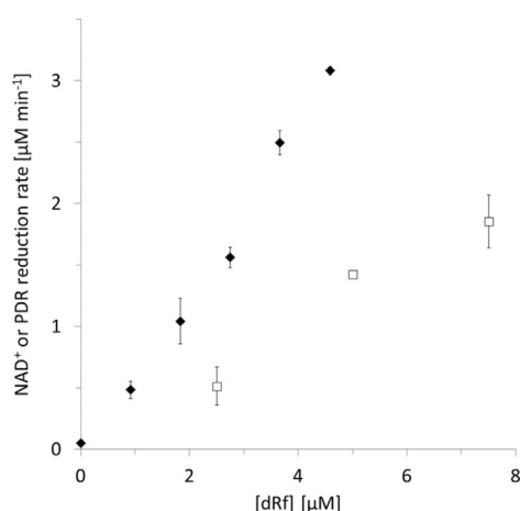
Figure 3. Rate dependency of the photoenzymatic reduction of NAD + (□) and the PDR (◆) on the dRf concentration applied. General conditions: Tris-HCl buffer (50 mM, pH 8), c(NAD + ) = 0.4 mM, c(EDTA) = 10 mM, c(PDR) = 2.5 (□) or 20 μM (◆), T = 25^{\circ}\text{C} , \lambda = 450\text{ nm} , anaerobic.
