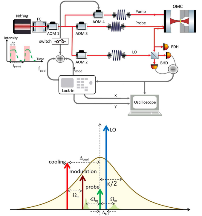
Fig. 2. Layout of the experimental setup (see text) and conceptual scheme of the field frequencies. The LO is placed on the blue side of the probe and detuned by \Delta_{\text{LO}} \ll \Omega_m , therefore the Stokes line is on the red side of the LO, while the anti-Stokes line is on its blue side. In the heterodyne spectra, they are located respectively at \Omega_m + \Delta_{\text{LO}} (Stokes) and \Omega_m - \Delta_{\text{LO}} (anti-Stokes).
