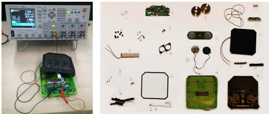
Figure 4: Measuring the power production of the PV cells and the power consumption, and an overview of components of the Eton Rugged Rukus speaker.
