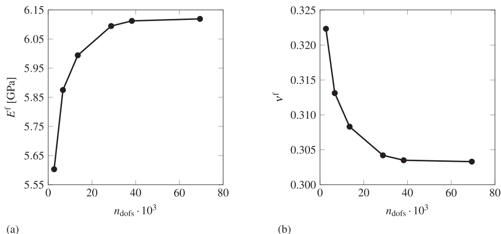
Fig. 8. Convergence of the estimated (a) E^f and (b) \nu^f with respect to the number of degrees of freedom n_{dofs} for an (8,8)-polymer composite.
