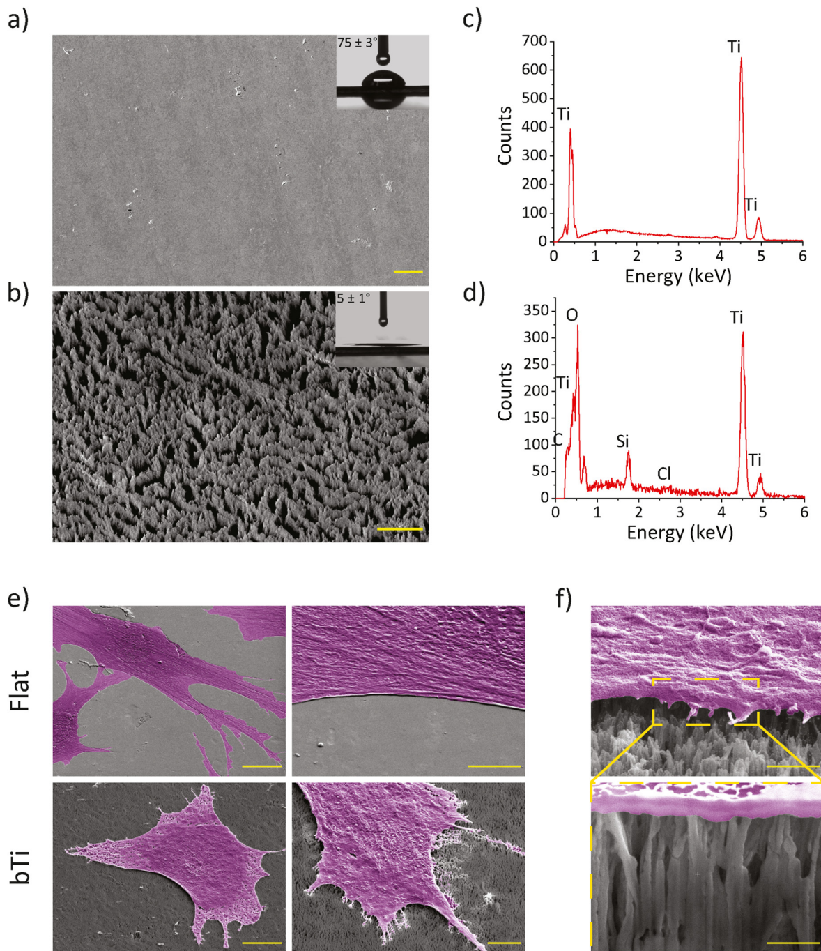
Fig. 2. a) A top-view SEM image of the polished Ti surfaces before the application of the ICP RIE process. The inset depicts the water droplet residing on the surface after 5 s. Scale bar = 20 \mu m. b) A tilted-view SEM image of the bTi surfaces made through ICP RIE. The inset depicts the water droplet residing on the surface after 5 s. Scale bar = 5 \mu m. EDS spectra of c) flat Ti and d) bTi surfaces, showing the most abundant chemical elements identified on each surface. e) The representative SEM images of hMSCs settled on the flat Ti and bTi surfaces for 1 day. Left column: low magnification images showing the cell morphology. Scale bar = 20 \mu m. Right column: higher magnification images showing the presence (absence) of filopodia around the cell periphery on the bTi (flat Ti) surfaces. Scale bar = 5 \mu m. f) A high magnification tilted view of the cell periphery in contact with high aspect ratio nanopillars, scale bar = 1 \mu m, and a cross-sectional view of the interface (shown by yellow dashed lines), scale bar = 500 nm. The cells have been false-colored for better visualization.
