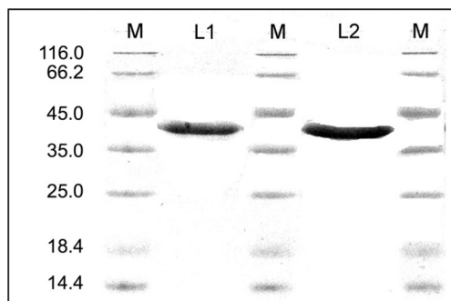
Fig. 3 SDS-PAGE analysis of FOYE-1 samples. M marker proteins, lane 1 purified FOYE-1 (5 \mu g protein), and lane 2 purified FOYE-1 (7.5 \mu g protein)
