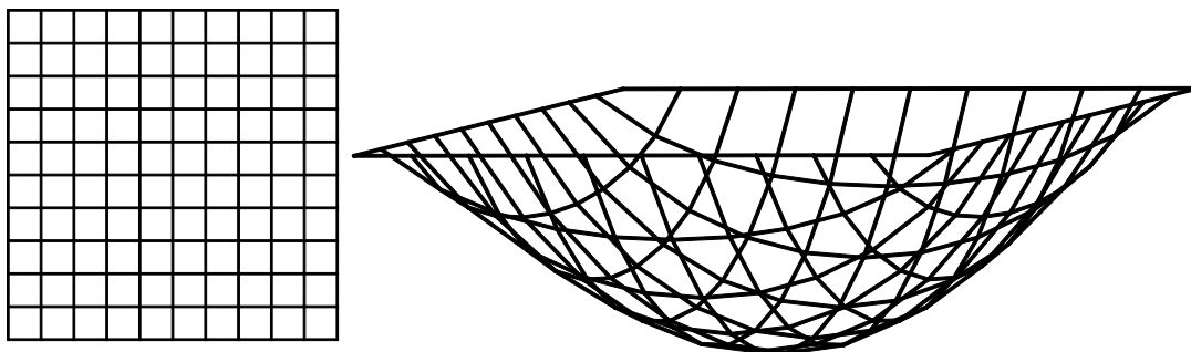
Figure 8: Hanging network with a force density of 2 of all elements supported in the boundary lines
