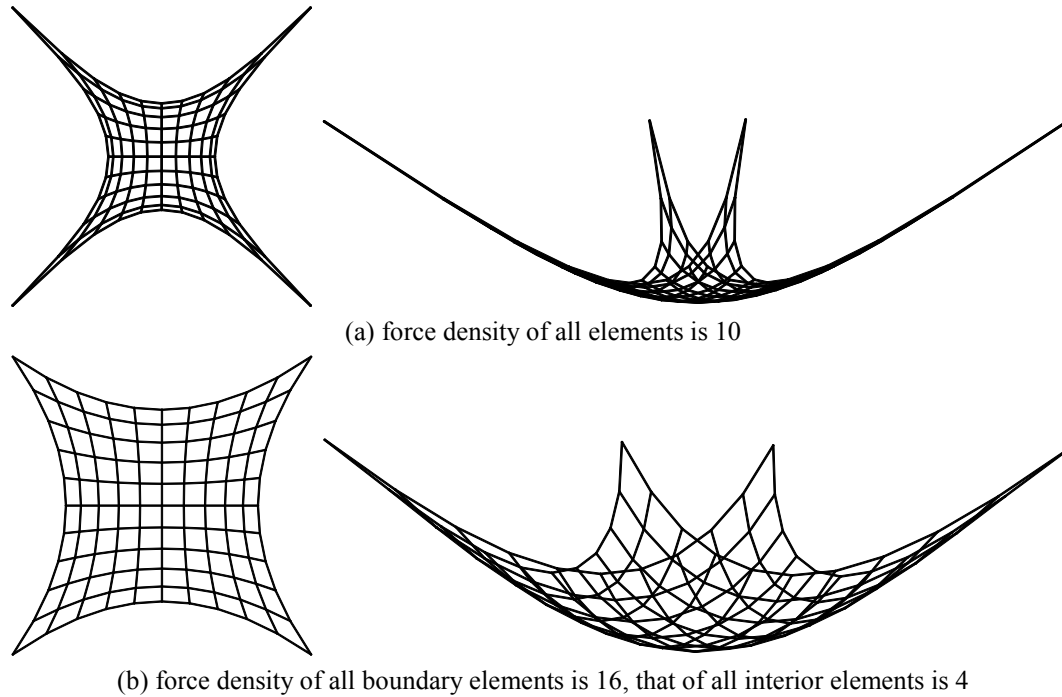
Figure 9: Hanging network supported in the corners
