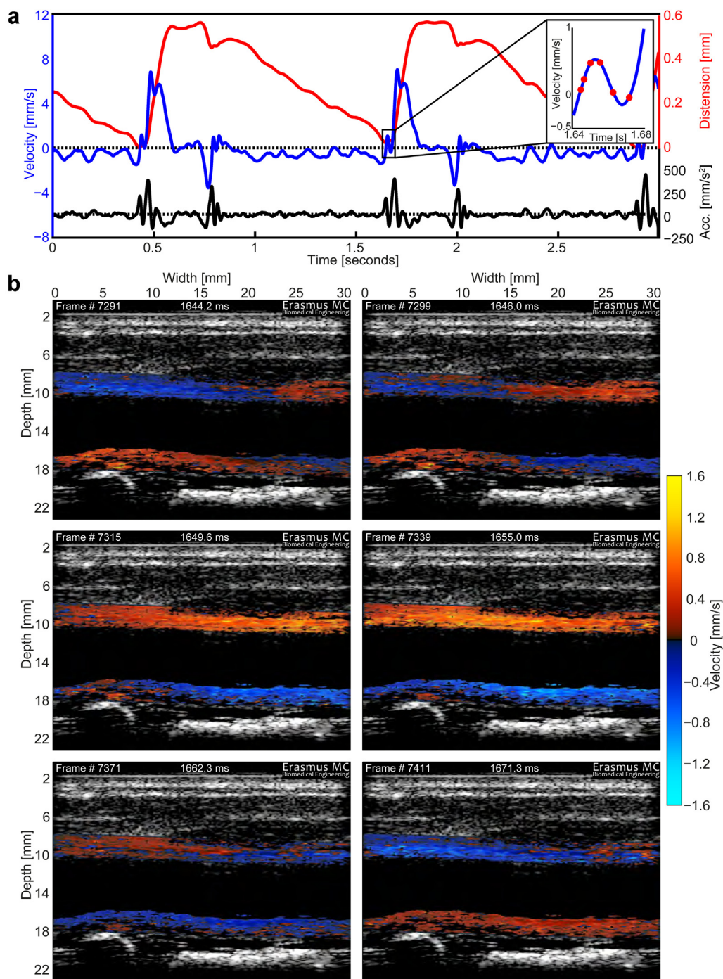
Fig. 7. Imaging transient phenomena along the arterial wall. The interaction of the pulse wave with the carotid artery wall can be visualized with high-frame-rate ultrasound imaging. This figure comprises six individual tissue velocity frames from a healthy carotid artery during a 27-ms episode. The pulse wave comes in from right to left. In (a) are distension waveforms of the same artery. Inset: Small magnified section of the distension waveform, where red dots indicate the frames below.
