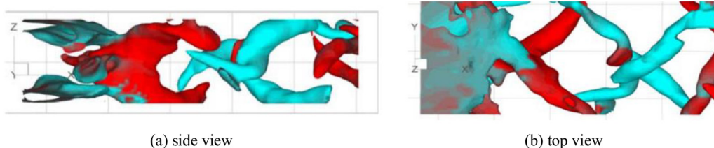
FIG. 13. Rhombus vortex cells at Re = 360 from (a) side view and (b) top view. Reproduced with permission from Scarano and Poelma, Exp. Fluids 47 , 69 (2009). Copyright 2009 Author(s), licensed under a Creative Commons Attribution Noncommercial License (CC BY-NC 2.0). 84
