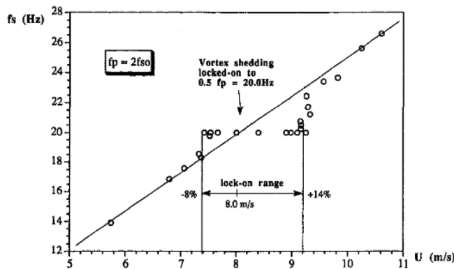
FIG. 38. Shedding frequency against the inflow velocity during the lock-on at F/F_{so} = 2 . Reproduced with permission from Wolochuk et al. , J. Fluids Eng. 118 , 18–25 (1996). Copyright 1996 The American Society of Mechanical Engineers. 188
