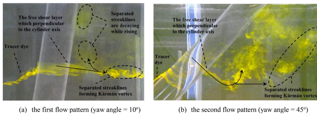
FIG. 17. Instantaneous wake patterns behind an inclined circular cylinder at Re = 5000 (a) yaw angle = 10^\circ , and (b) yaw angle = 45^\circ . Reproduced with permission from Najafi et al. , Ocean Eng. 113 , 335–349 (2016). Copyright 2016 Elsevier. 104
