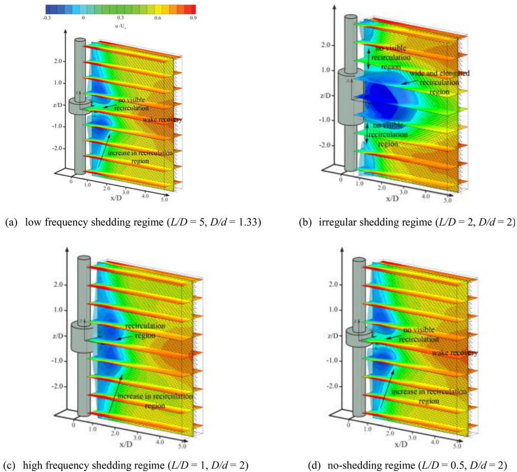
FIG. 37. Planar contours of the mean streamwise velocity behind a dual-step cylinder at Re = 2000 (a) low-frequency shedding regime, (b) the irregular shedding regime, (c) high-frequency shedding regime, and (d) no-shedding regime. Reproduced with permission from Morton et al. , Phys. Fluids 28 , 025104 (2016). Copyright 2016 AIP Publishing LLC. 186
